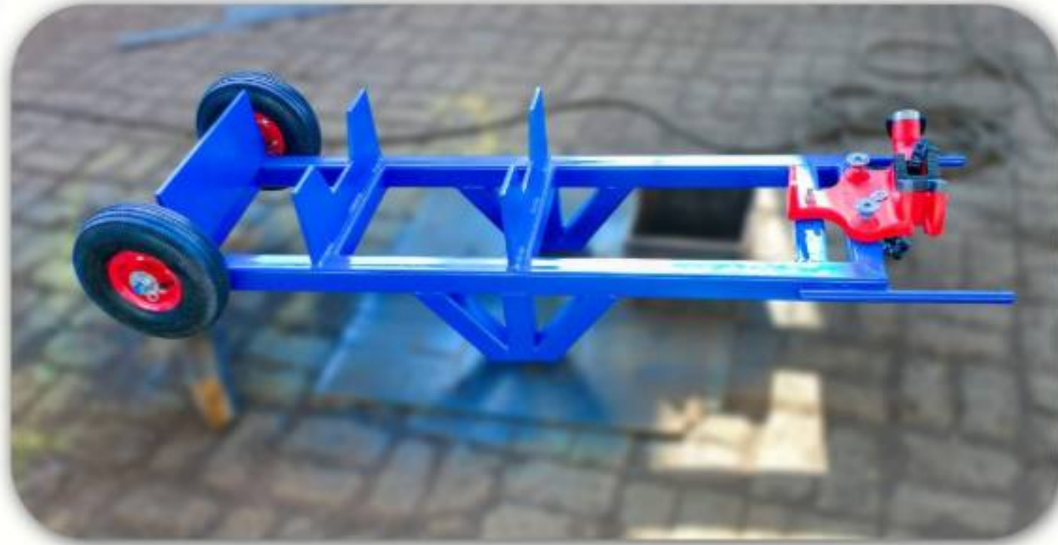
Tool Trolley
